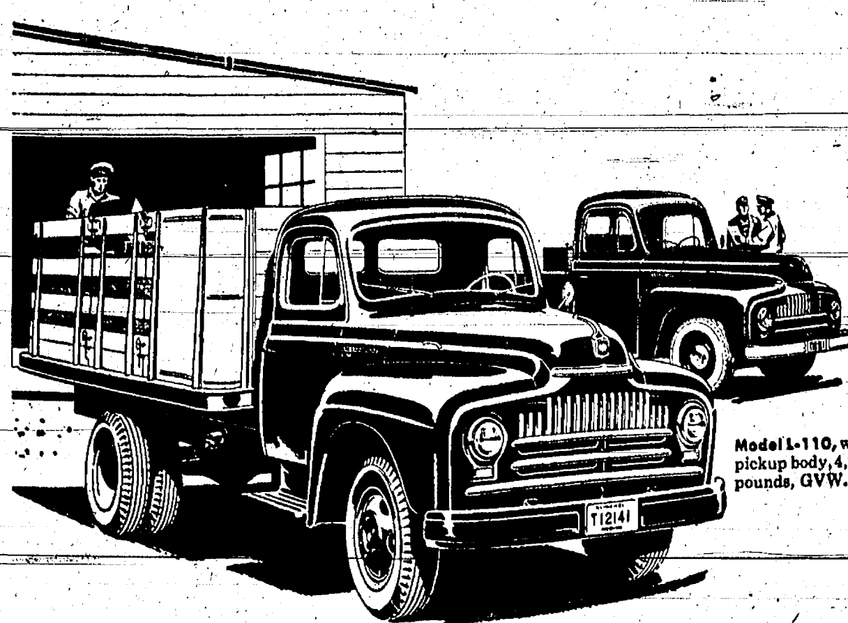
Model L-160, 164-inch wheelbase, 12-foot stake body, 14,000 lbs. GVW, featuring: Comfort-Vision Cab, Silver Diamond 240 engine, 4-speed Synchronesh transmission, 37° turning angle, roller-mounted steering gear.
